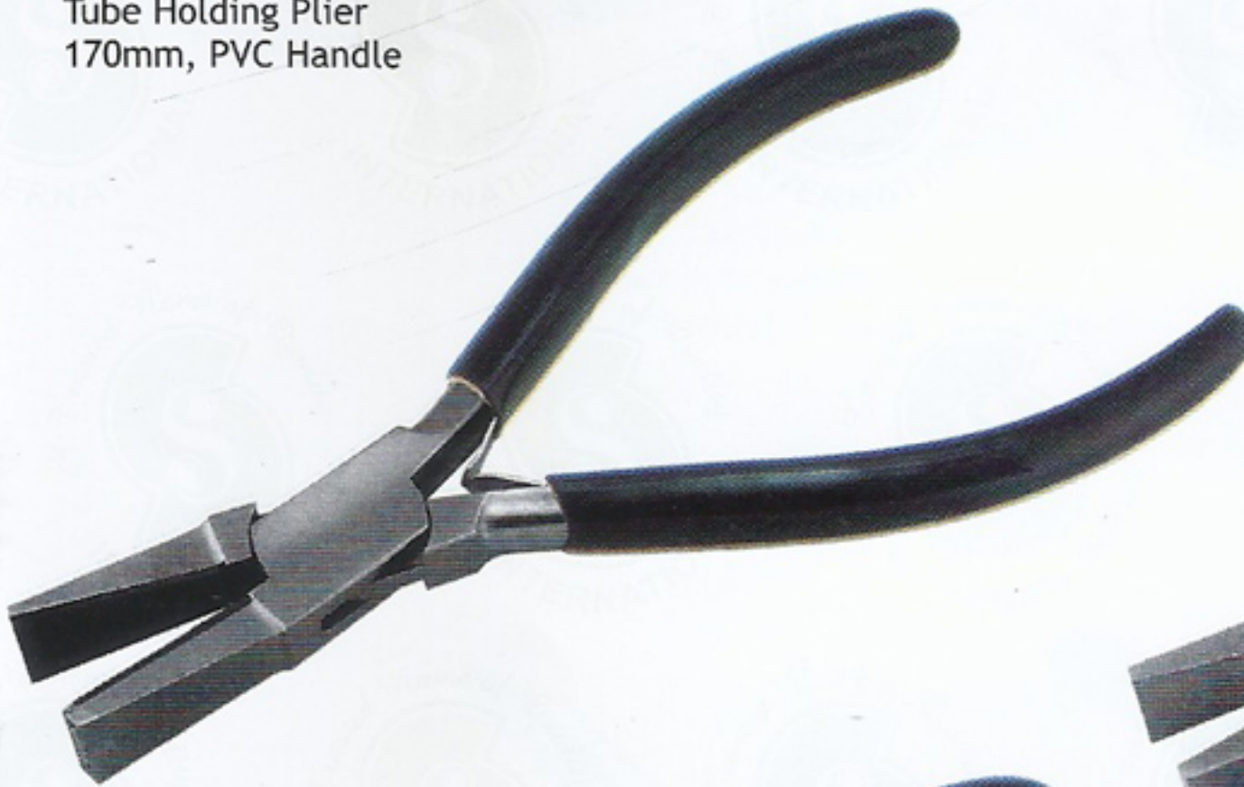
PLR1642-SI Duckbilled Plier, 170mm With Urthane Jaw Pvc Handle with Spring
