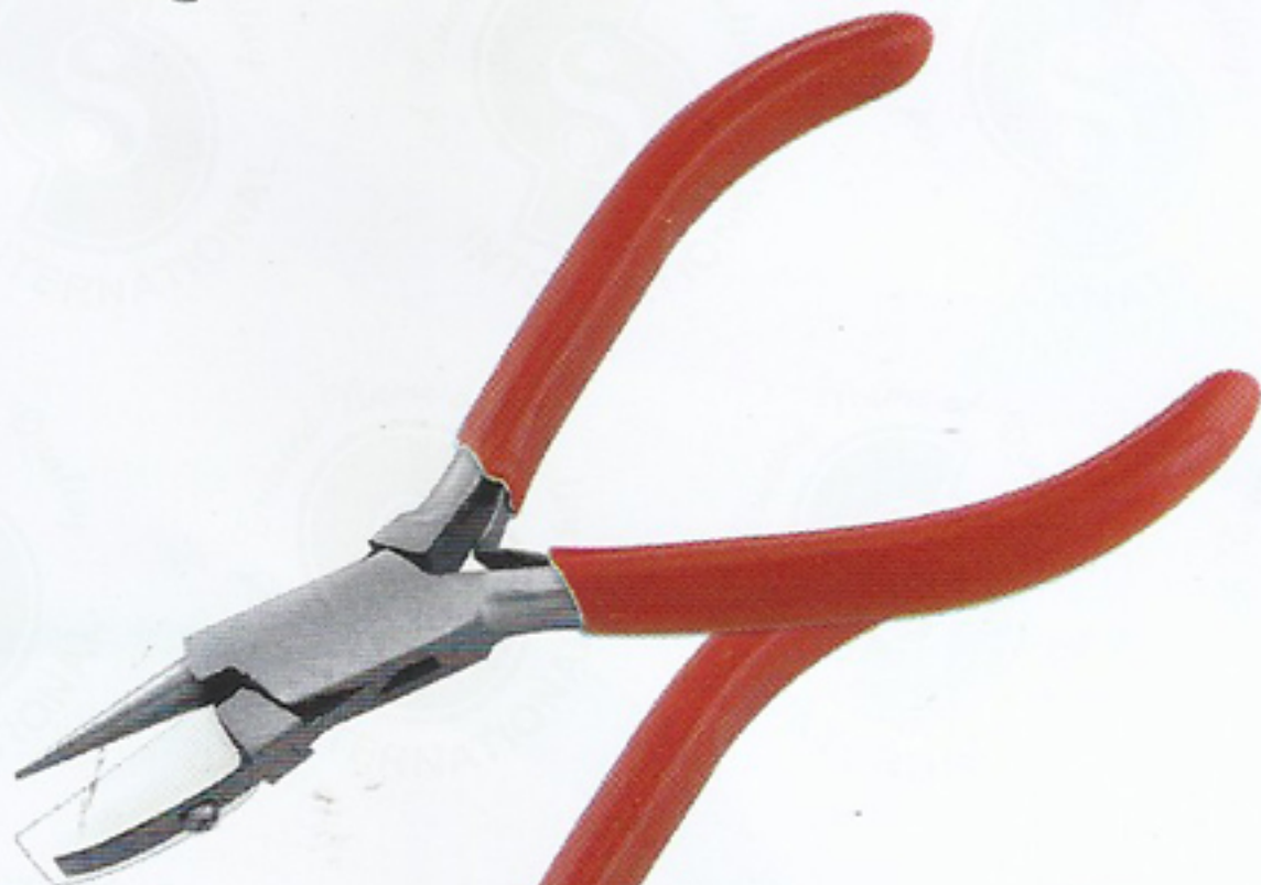
PLR1751-SI Round Nylon Jaw Plier 120mm, Leaf Spring Pvc Handle
